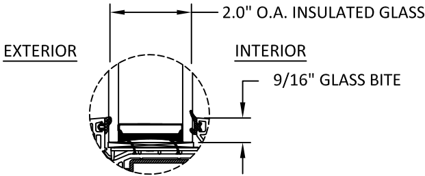
GLAZING DETAIL 1
